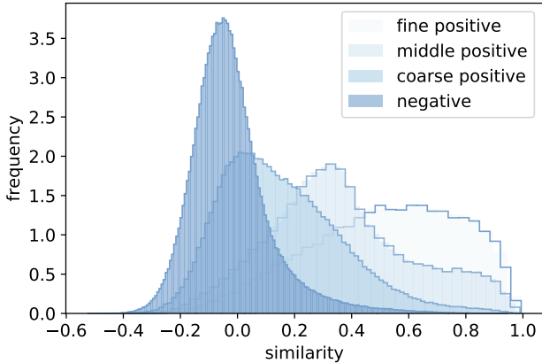
Figure 5. The distribution of similarity scores indicates conflicts between different scales.
