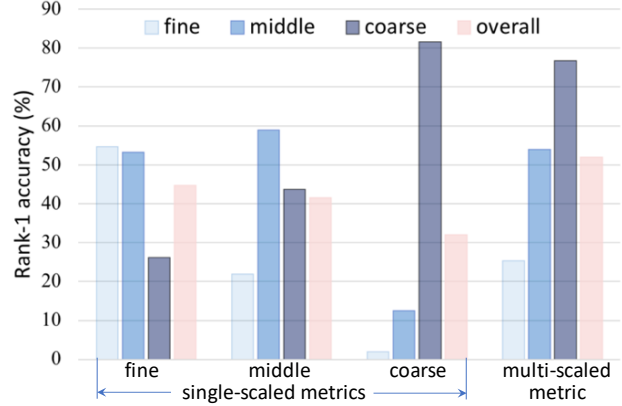
Figure 4. Comparison between single-scaled metrics and a multi-scaled metric baseline on DyML-Animal. The multi-scaled metric surpasses all the single-scaled metrics on the overall accuracy.
