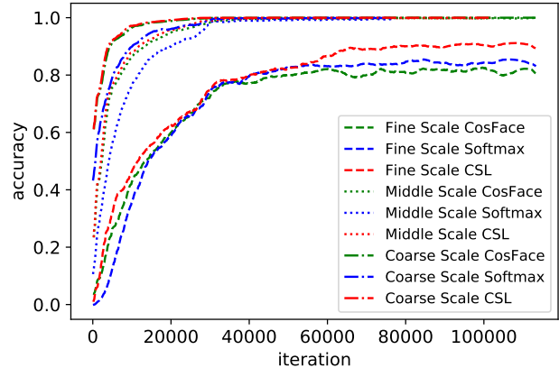
Figure 6. Comparison between the training process of softmax, cosface and CSL on DyML-Animal. Compared with the multi-scale learning baselines, CSL obtains faster convergence and higher classification accuracy on the training set, because it alleviates the mutual conflict between different semantic scales.
