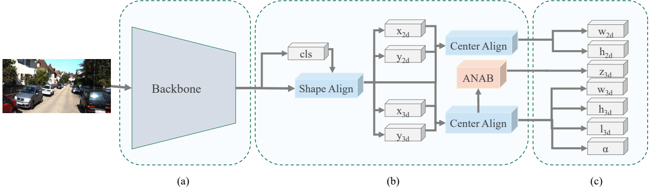
Figure 1: The architecture of M3DSSD. (a) The backbone of the framework, which is modified from DLA-102 [43]. (b) The two-step feature alignment, classification head, 2D/3D center regression heads, and ANAB especially designed for predicting the depth z_{3d} . (c) Other regression heads.
