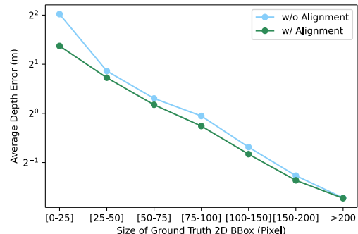
Figure 7: The average depth estimation error varies along with the size of objects that is the average of the length and the width of the 2D BBox. Best viewed in color.
