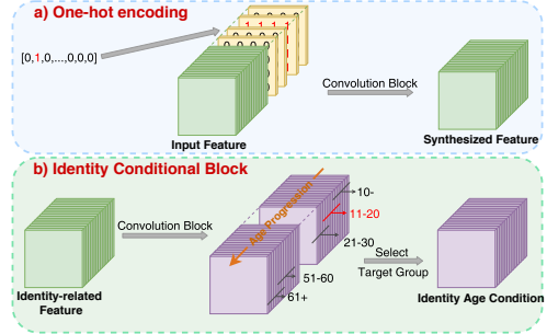
Figure 3: Comparison between one-hot encoding and ICB.
